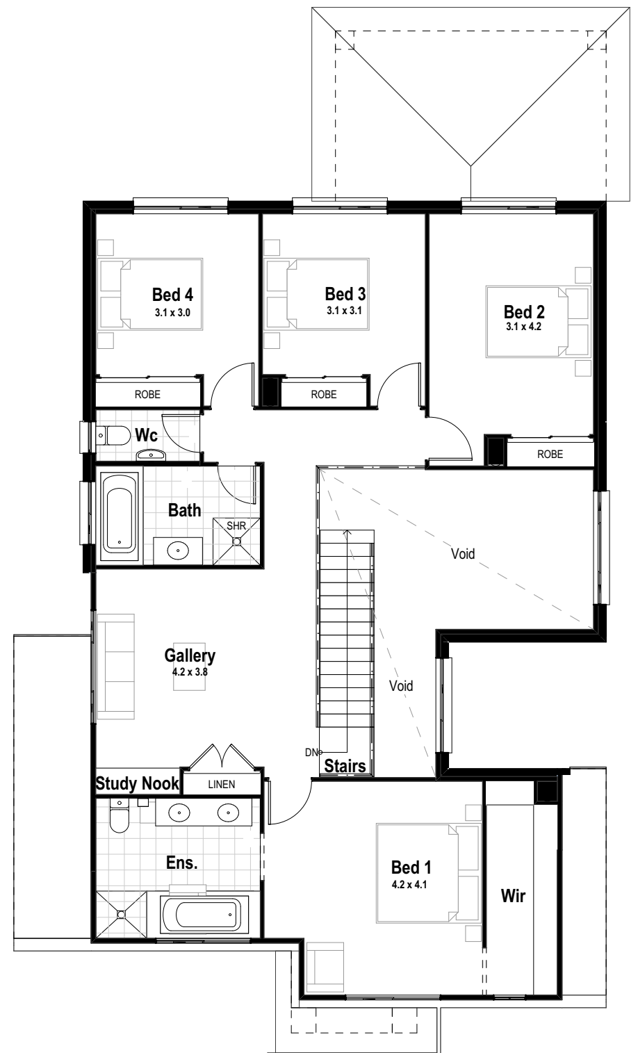
FIRST FLOOR
